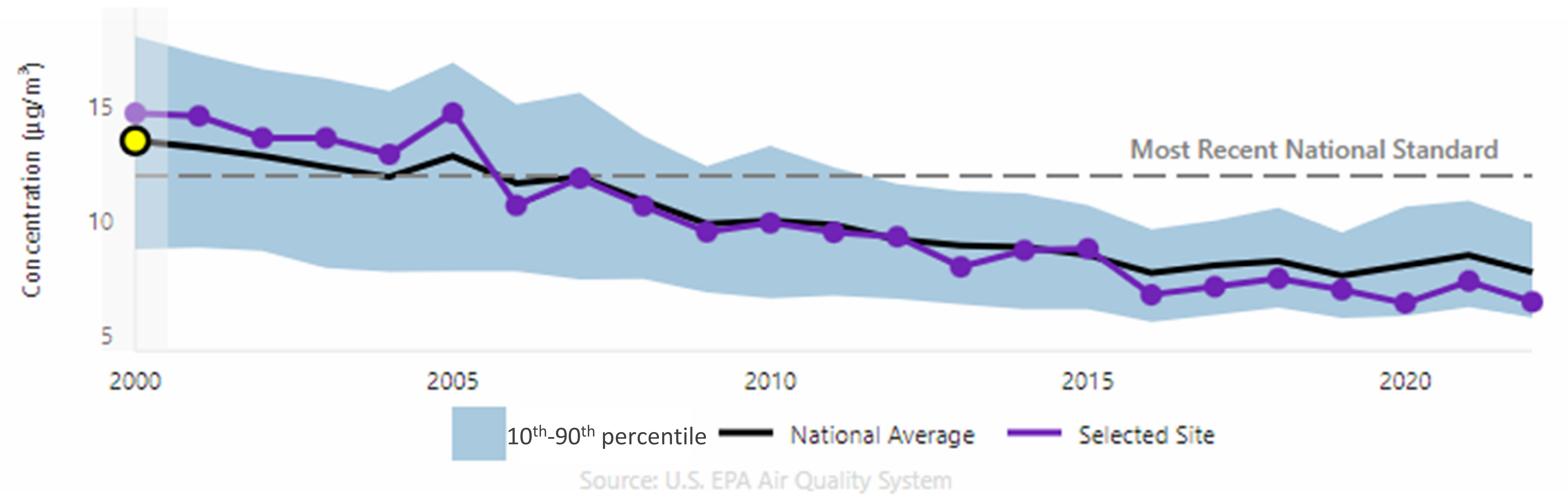
PM 2.5 Annual Concentration
