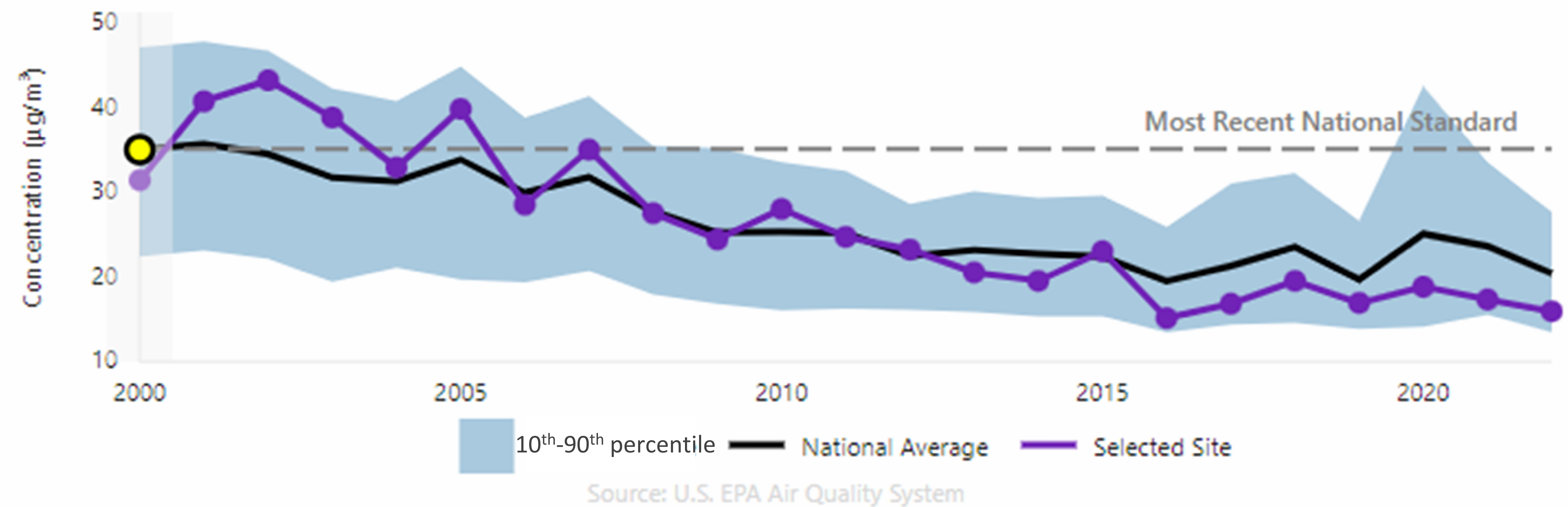
PM 2.5 24-hour Concentration
